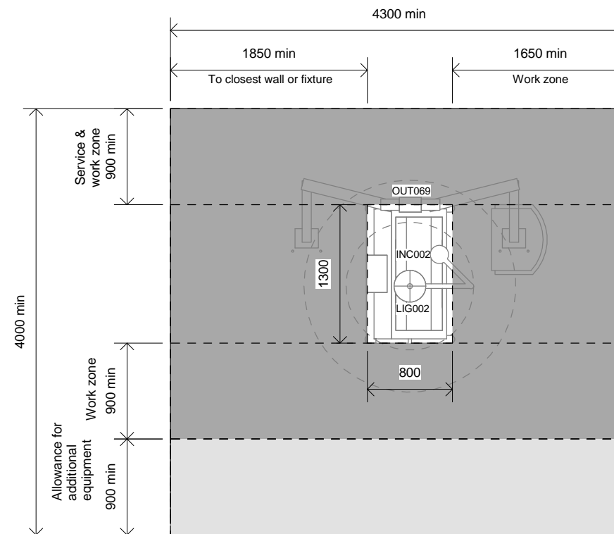
2 PLAN - INTENSIVE CARE TERTIARY 1 : 50
