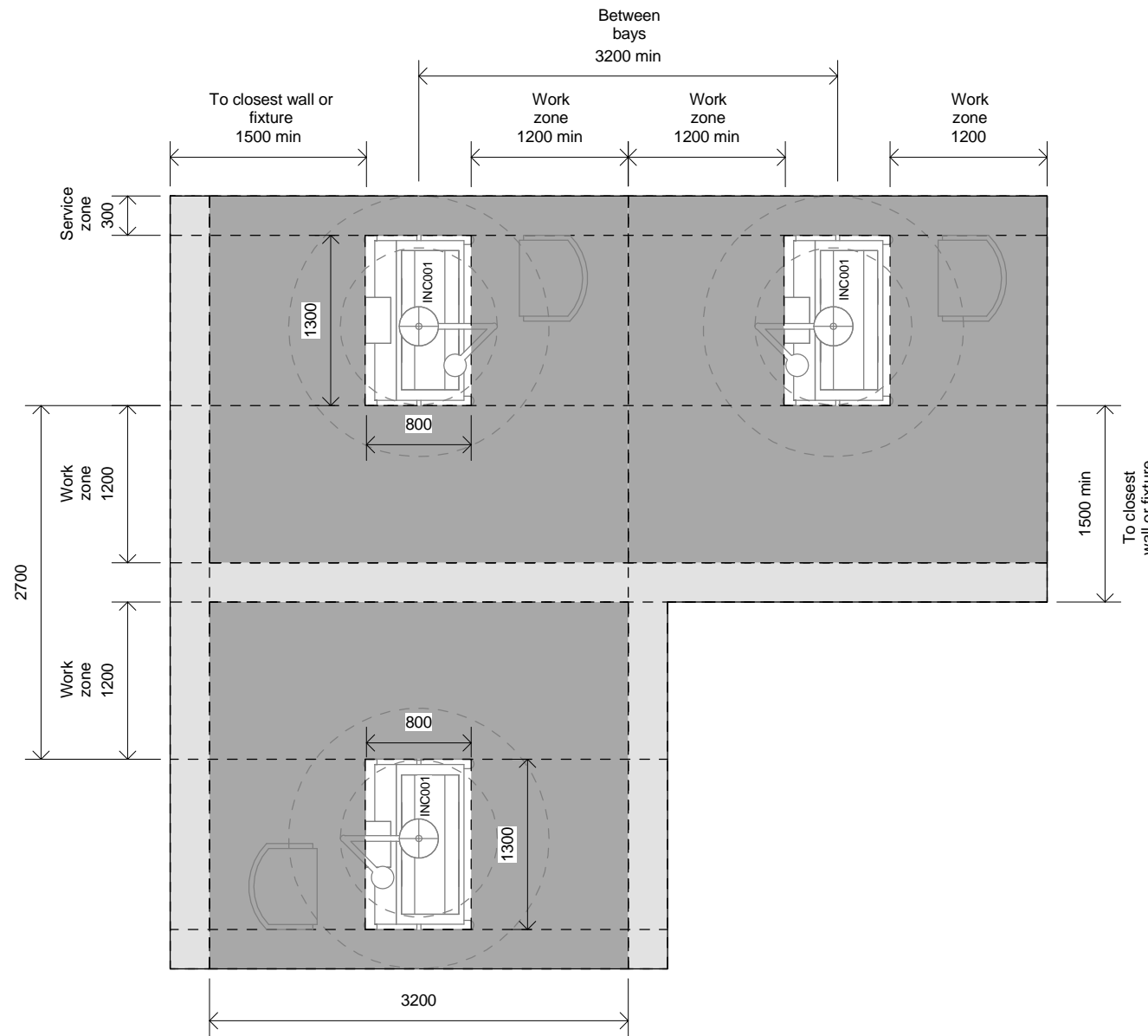
2 PLAN - HIGH CARE (INCUBATORS & BABY STATIONS) 1 : 50
