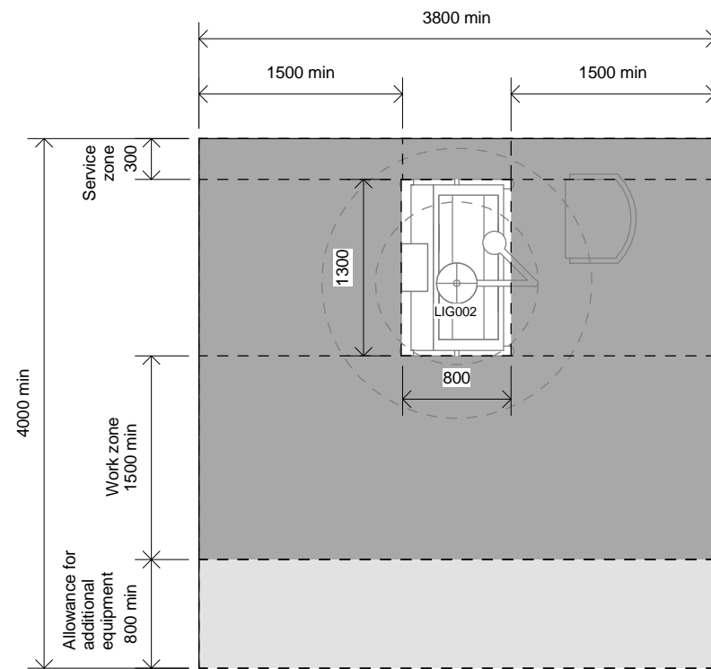
1 PLAN - INTENSIVE CARE STANDARD 1 : 50
