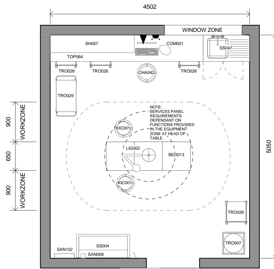
2 PLAN - PROCEDURE ROOM - STANDARD 1 : 50
