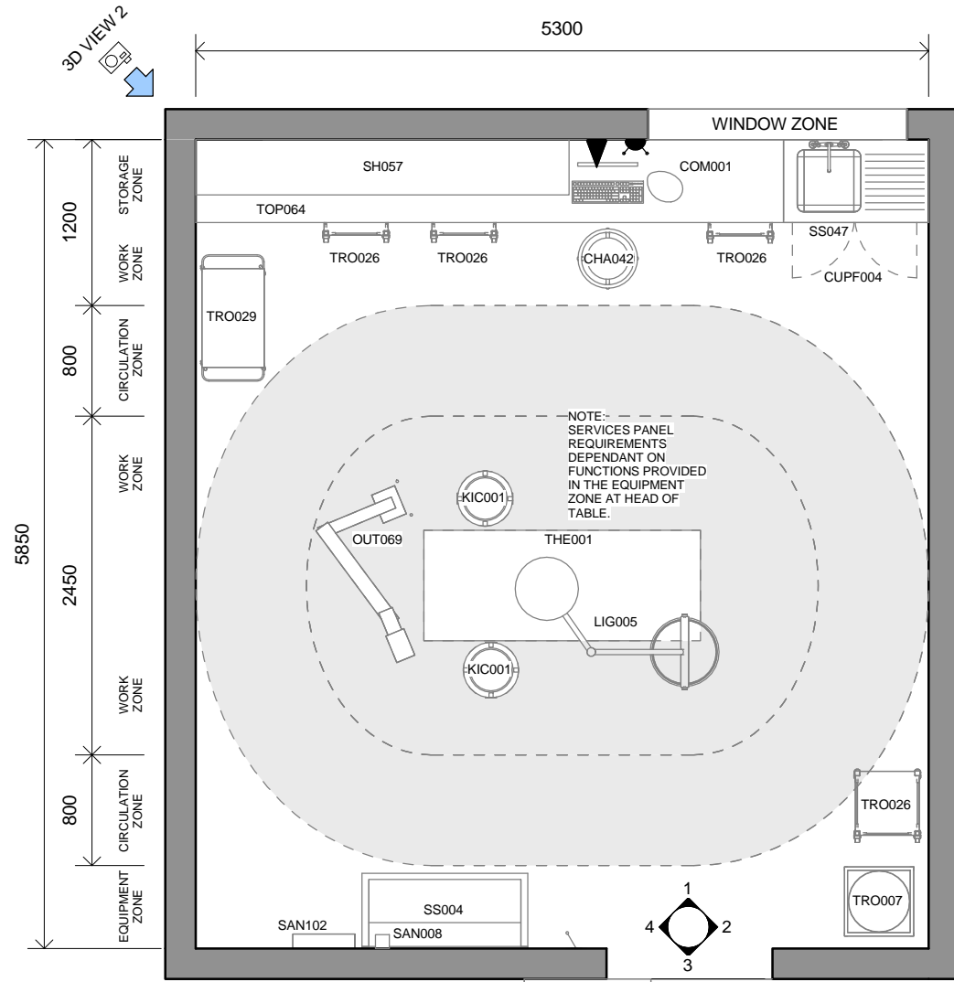
1 PLAN - PROCEDURE ROOM - EMERGENCY 1 : 50
